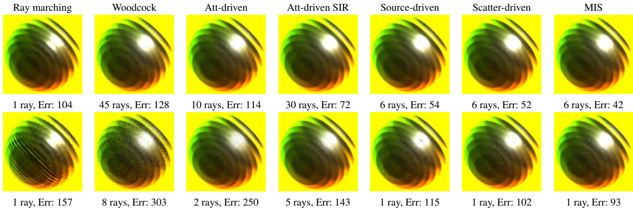
Figure 12: Equal number of medium parameter evaluations comparison of the proposed single scattering methods to classical single ray per pixel, constant step ray marching and multi-ray per pixel Woodcock tracking. Each method took approximately 300 samples (upper row) and 50 samples (lower row) from the medium per pixel on average to compute all primary and shadow rays. For each method, we show the number of primary rays requiring the same number of medium fetches, and the RMS errors.
