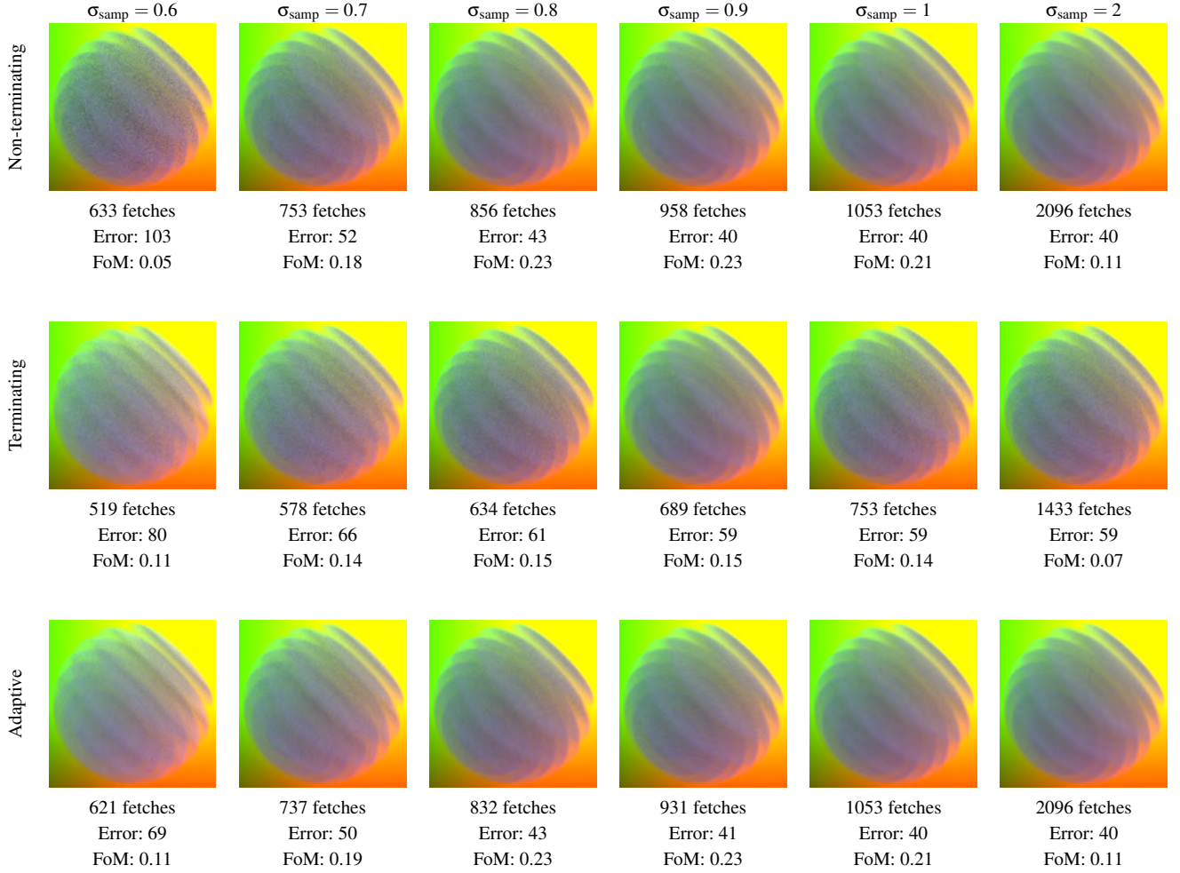
Figure 6: Particle tracing of the medium of Equation 21 with 100 rays per pixel setting the \sigma_{\text{samp}} value differently to demonstrate the effect of the sampling density on the number of volume fetches, i.e. the rendering cost, and on the rendering error. Increasing \sigma_{\text{samp}} reduces the variance until \sigma_{\text{samp}} < \sigma_l \leq \sigma_{\text{max}} = 1 on the ray as suggested by the variance analysis of the Single Particle Model in Section 3.4. However, the number of fetches becomes proportional to \sigma_{\text{samp}} , thus the sampling cost increases. The FoM efficiency metric is defined as the reciprocal of the product of the mean square error and the cost. Note that we do not require the sampling density to be a majorant, but its appropriate choice is still important as it affects the error-cost trade-off. In this case, the optimum value is \sigma_{\text{samp}} \approx 0.8 , which is below the maximum extinction, depending on the actual extinction values a given ray can see and also on the variation of the extinction and illumination inside a pixel. If the sampling extinction is too low, the variance grows rapidly, so the estimator becomes poorer.
