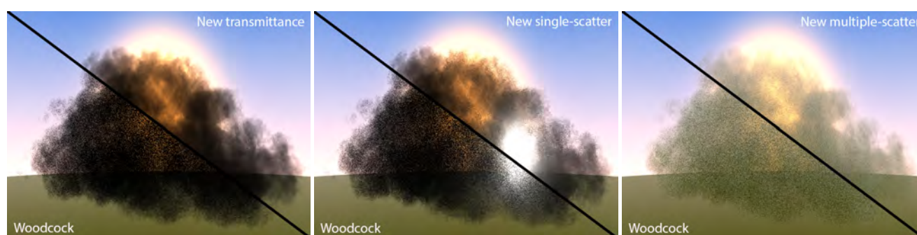
Figure 1: Transmittance (left), single-scatter of a point light source (middle), and multiple-scatter (right) calculation for 12-octave Perlin-noise medium and comparison to Woodcock tracking with equal number of medium fetches.
