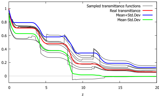
Figure 8: Sample transmittance functions on the ray going through the center of the analytic medium, the real transmittance, and probabilistic lower and upper bounds using the standard deviation that is the square root of the variance obtained with Equation 16. The real extinction and its main part are shown by the lower image of Figure 5, and the sampling extinction is \sigma_{\text{samp}} = 0.4 .
