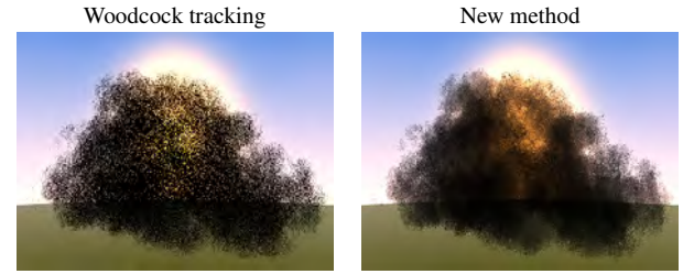
Figure 10: Comparison of the proposed transmittance estimation to Woodcock tracking. Each method took 20 samples from the medium density per pixel on average.
