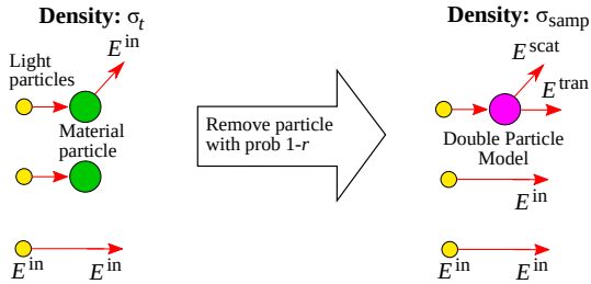
Figure 4: Randomly removing real particles decreases the density but preserves the expected radiance if interaction rules are simultaneously modified.
