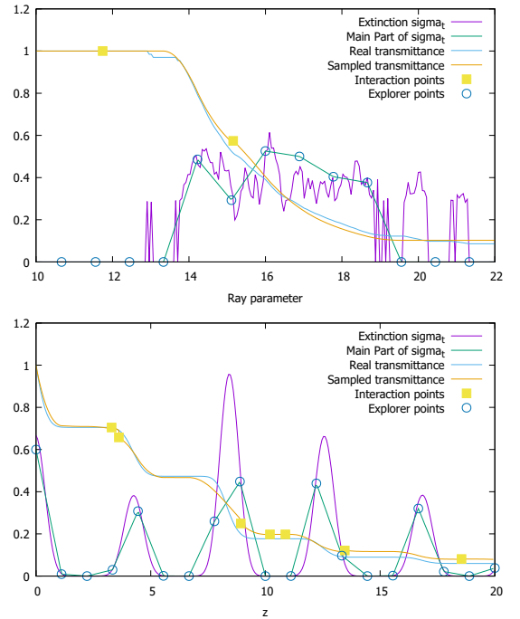
Figure 5: The anatomy of the ray going through the center of the Perlin-noise (top) and analytic medium (bottom) used in the experiments. We show one set of explorer points and random interaction points that together define one random sample of the complete transmittance function. Explorer points show where the approximate extinction is evaluated to obtain the control variate. Interaction points are generated when jumping on the ray with free flight distances to estimate the transmittance of the difference extinction. Sampling extinction \sigma_{\text{samp}} is 0.4 for this ray in the analytic medium.
