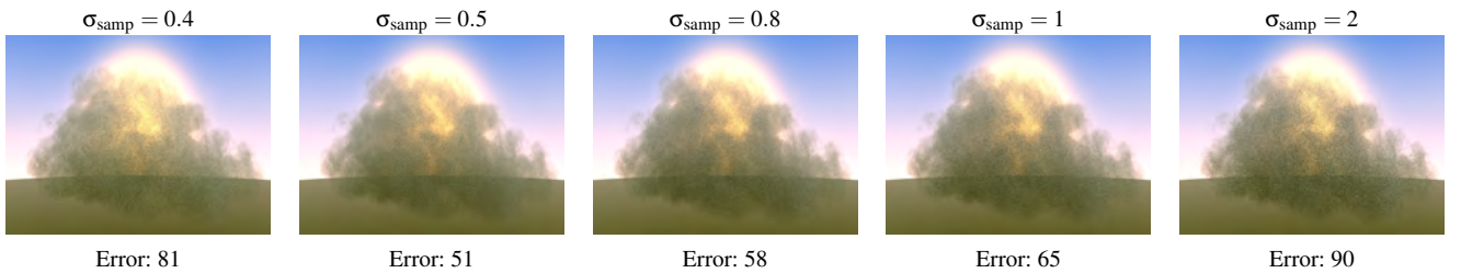
Figure 7: Particle tracing of a twelve-octave Perlin noise with equal number of medium parameter evaluations, i.e. equal cost, setting sampling density \sigma_{\text{samp}} value differently. The extinction is evaluated 500 times per pixel in each method. The optimal \sigma_{\text{samp}} value is slightly below the extinction of the larger dense regions. In this medium, the maximum of the extinction is 1, but most of the rays meet extinctions less than 0.6.
