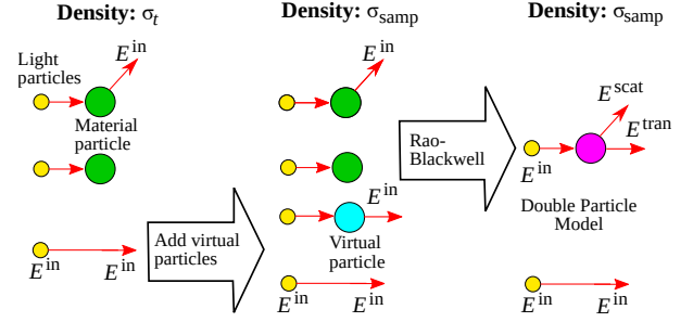
Figure 2: Adding virtual material particles of Dirac-delta phase function and albedo 1 increases the medium density but preserves the expected radiance. Rao-Blackwellization replaces the three random cases of scattering, transmission and absorption by weighting.
