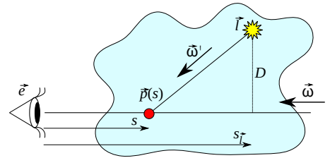
Figure 11: Single scattering of point source lighting.
