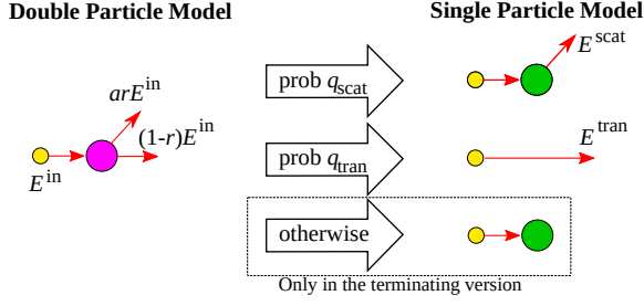
Figure 3: The Single Particle Model is the randomization of the Double Particle Model. Randomization is the inverse of Rao-Blackwellization, but can use different probabilities. Only the terminating version allows particles to be absorbed.
