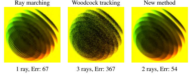
Figure 9: Equal number of medium parameter evaluations comparison of the proposed transmittance estimation to classical single ray per pixel ray marching and multi ray per pixel Woodcock tracking. Each method took 10 samples from the medium density per pixel on average.
