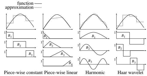
Figure 56: Basis function systems and finite-element approximations
