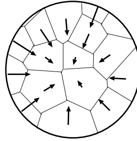
Figure 15: Radiance values of texels within the Voronoi areas are summed to compute their total power and the final Delaunay grid on high dynamic range image. The centers of Voronoi cells are the sample points.
