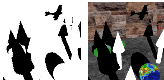
Figure 8: Hardware shadow mapping with 512 \times 512 shadow map resolution at 210 FPS.
