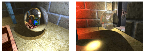
Figure 44: Reflective and refractive spheres in a game environment (105 FPS)
