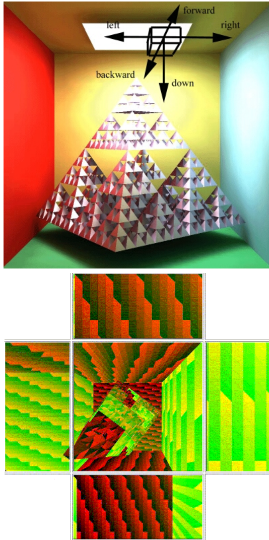
Figure 4: Placement of the hemicube around a lightsource point and the images on the 5 hemicube faces
